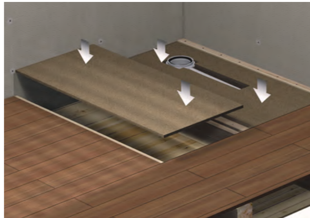
4. Fix timber panels to support ensuring a level deck at joist height.
