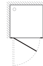
Door opening
