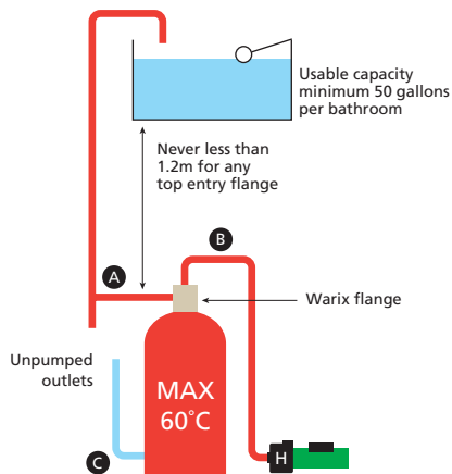
Figure 30: Approved flanges
