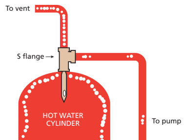
Figure 29: S flange
