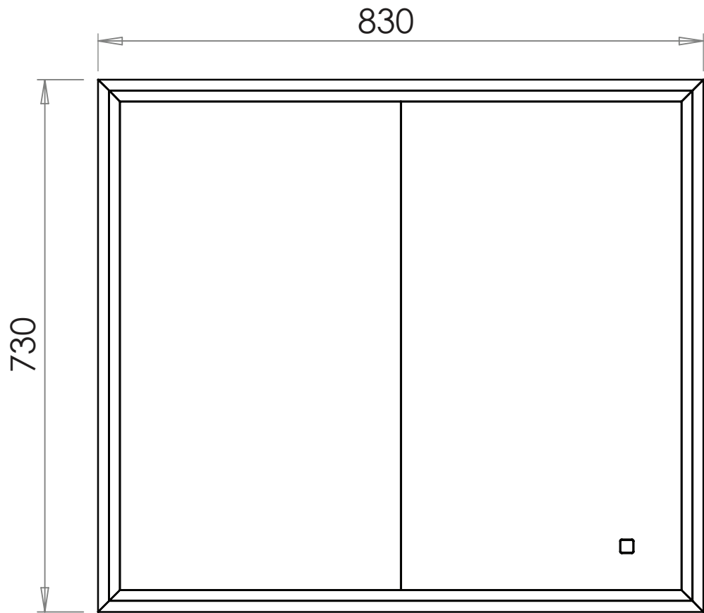
External Cabinet Dimensions
