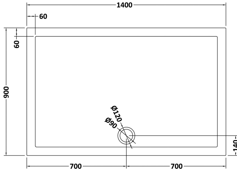
NTP034 - 1400 x 900 RECTANGULAR TRAY
