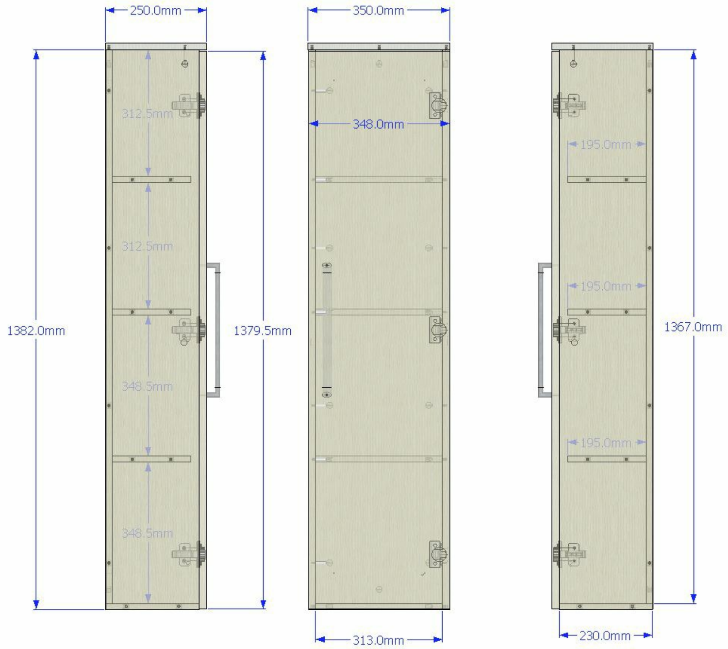
Left Elevation
